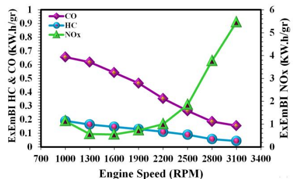
Figure 18: ExEmBI HC, CO and NOx at various engine speeds.
