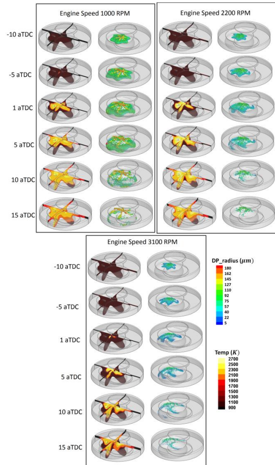
Figure 6: Droplet size distribution and Combustion temperature contours for different engine speed 1000 RPM, 2200 RPM and 3100 RPM
