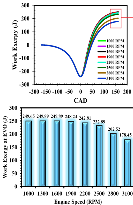
Figure 12: Work exergy variation with respect to CAD and EVO for different engine speed.
